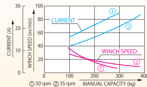
• RES-4024, REL/RES-4024 (400 W, 24 V Type)
