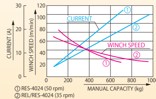
• RES-4024, REL/RES-4024 (400 W, 24 V Type)
