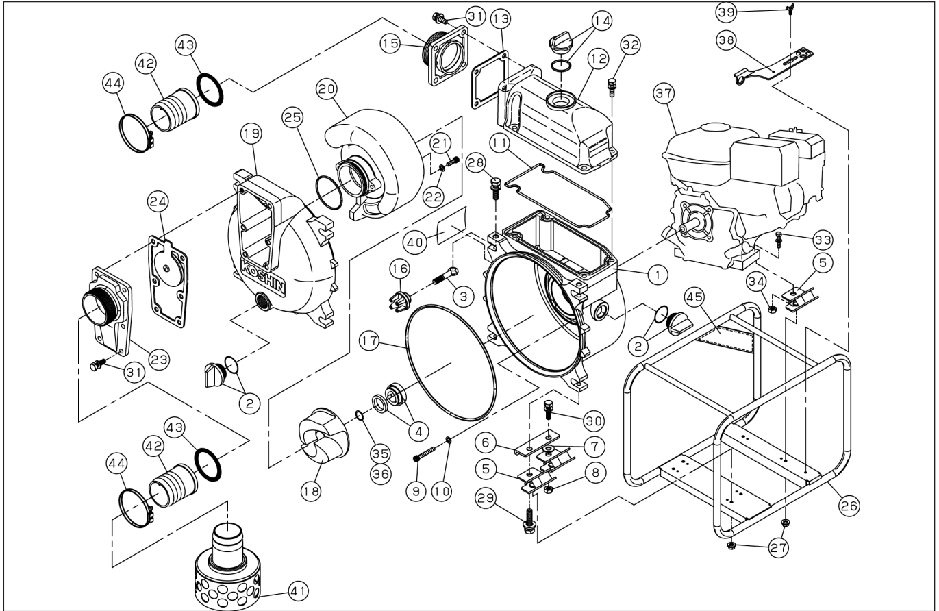
DWG No.013858201 MODEL : KTH-100X FORM : KTH-100X-BAR-0 (GX340UT2)
