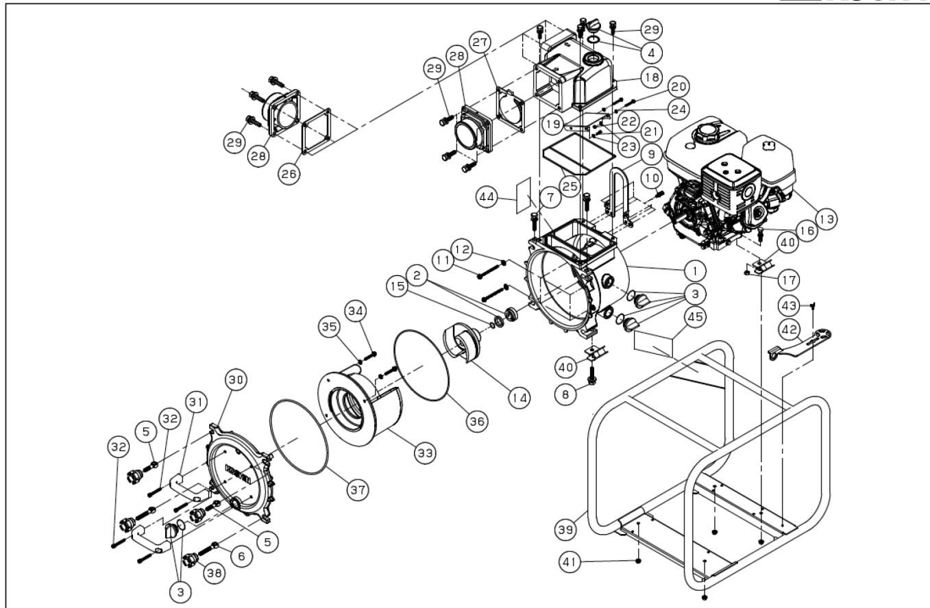
DWG No.012A12801 MODEL : KTH-80S FORM : KTH-80S-BAL-0(GX270)
