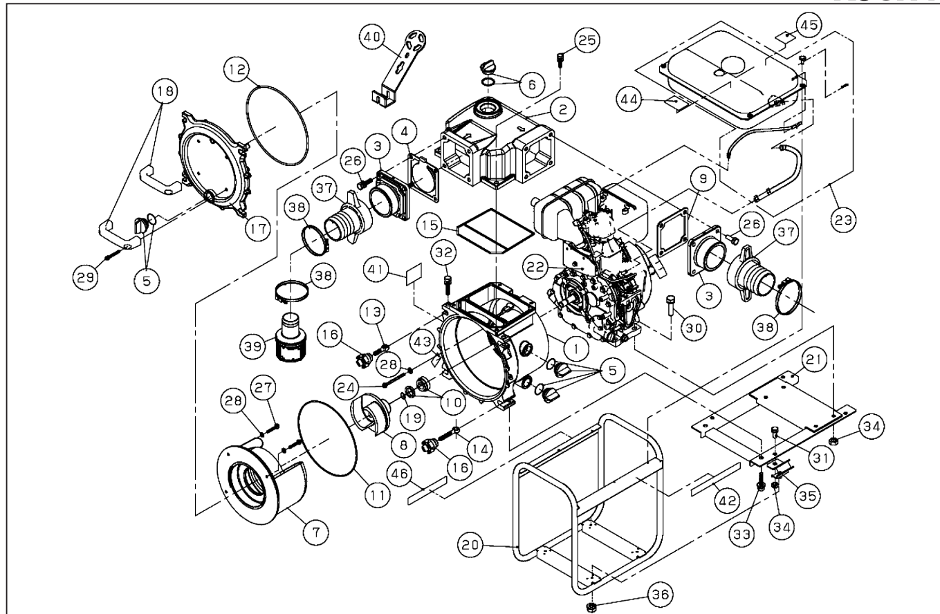
DWG No.012943404 MODELE : KTY-100D FORM : KTY-100D-BAB-0
