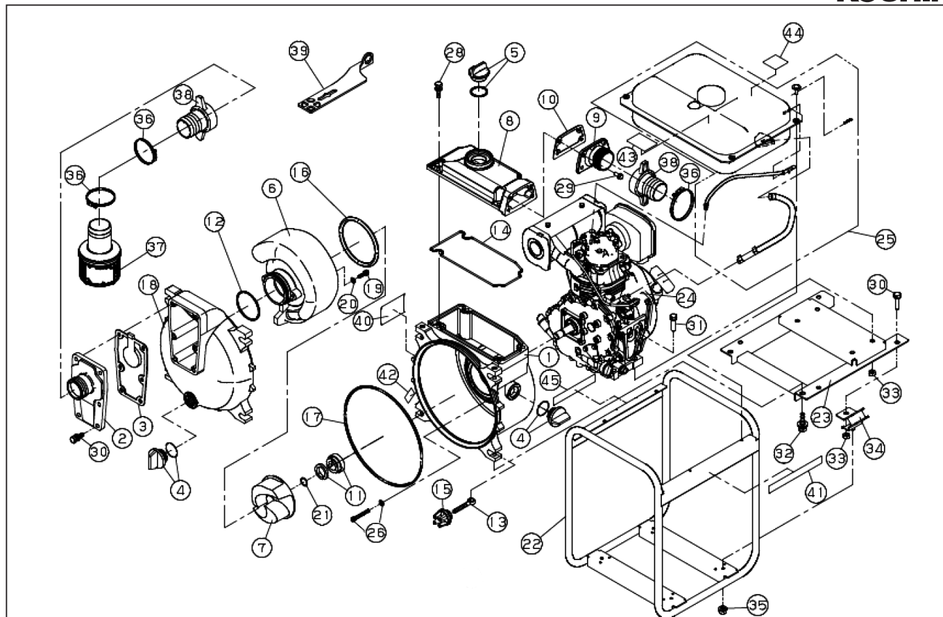
DWG No.012943201 MODELE : KTY-50D FORM : KTY-50D-BAB-0
