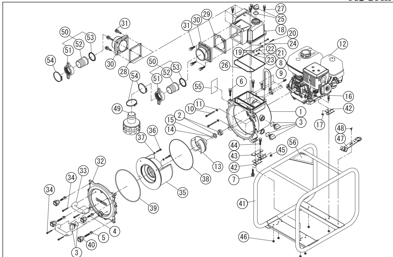
DWG No.012948401 MODELE : KTZ-100S FORM : KTZ-100S-BAA-0(K420)
