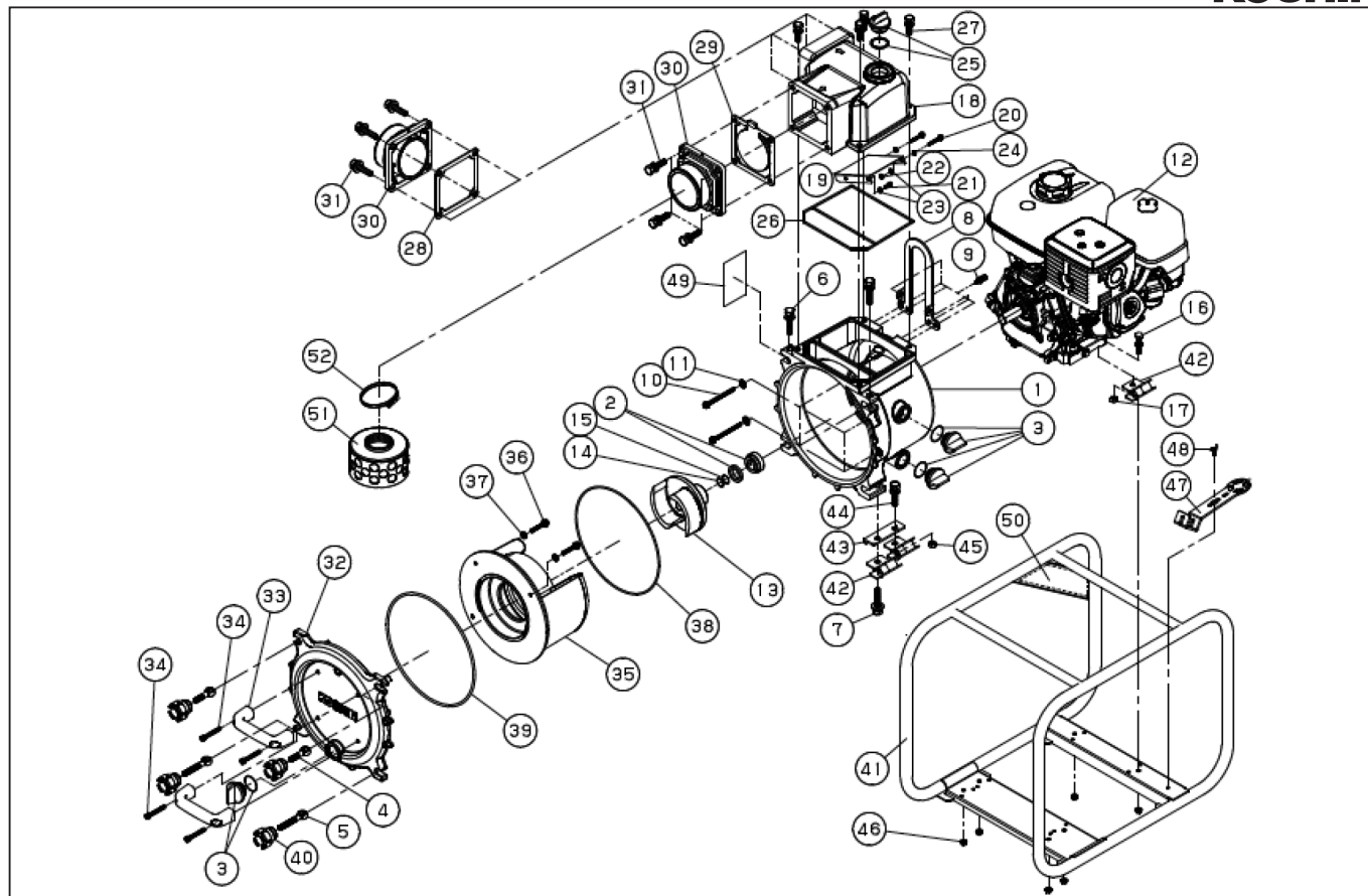
DWG No.012948604 MODELE : KTZ-100S FORM : KTZ-100S-BAB-1(K420)
