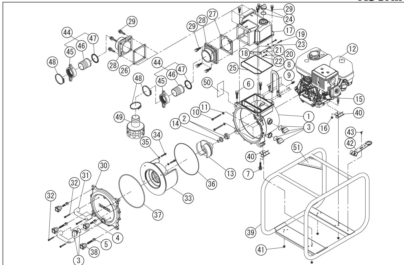
DWG No.012948301 MODELE : KTZ-80S FORM : KTZ-80S-BAA-0(K300)
