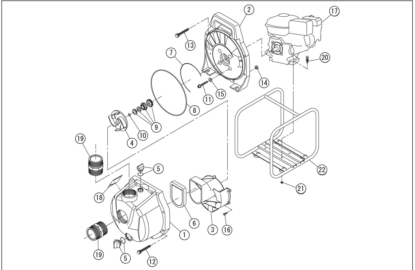
DWG No.013850308 MODELE : PGH-50 FORM : PGH-50-BAC-1
