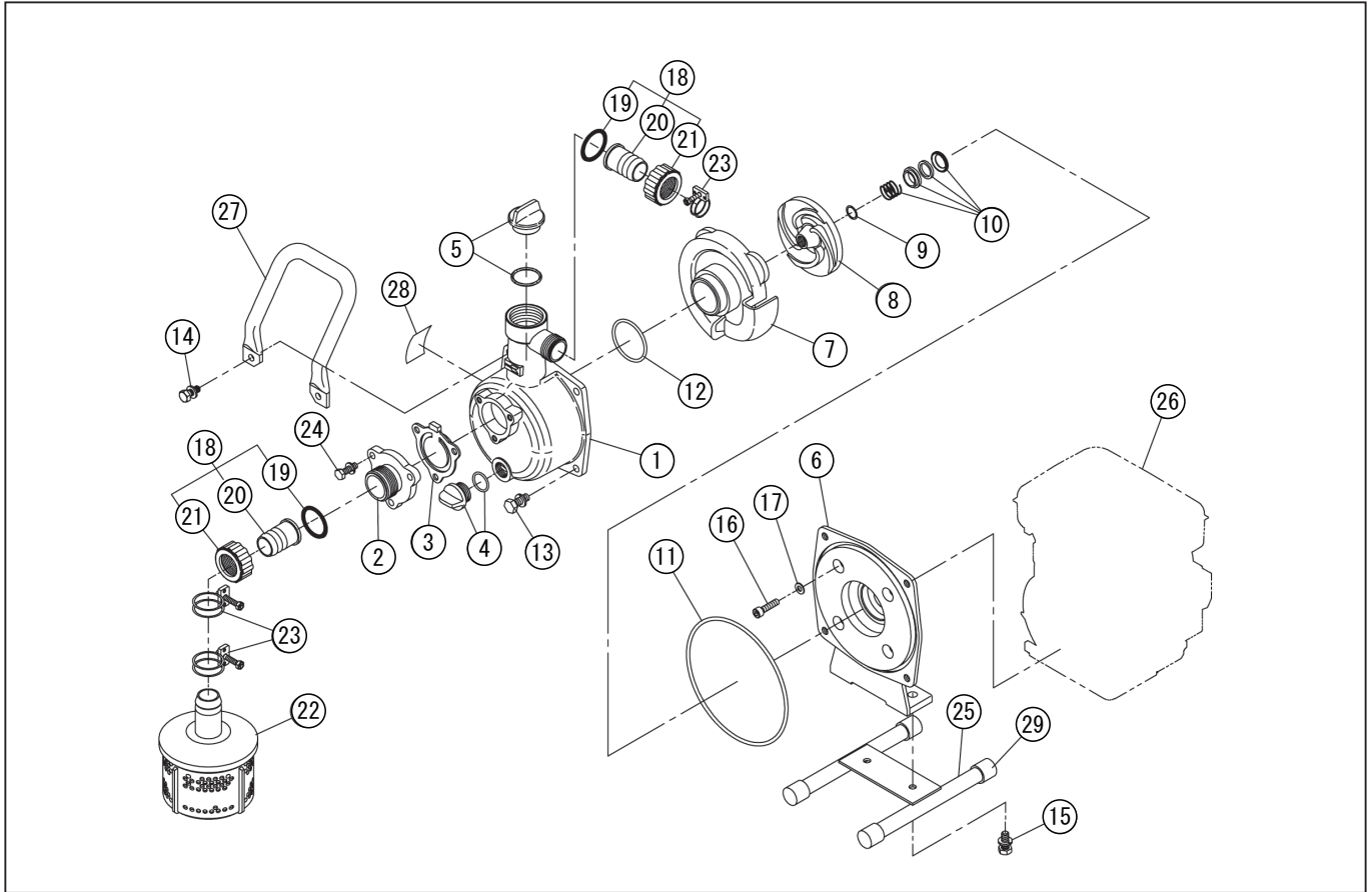
DWG No.012875804 MODEL : SE-25F FORM : SE-25F-BAD-0
