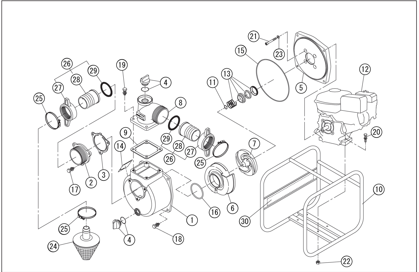
DWG No.012897408 MODEL:SE-50EX FORM:SE-50EX-BAJ-3
