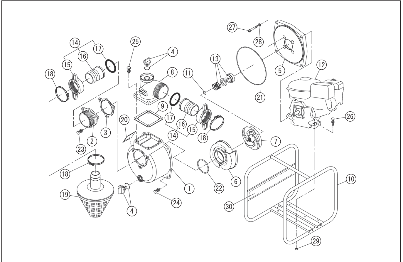
DWG No.066865301 MODEL : SE-50X FORM : SE-50X-BDY-0 (EY15-3)
