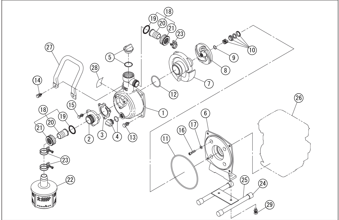
DWG No.012919701 MODELE : SEH-25L FORM : SEH-25L-BAF-0
