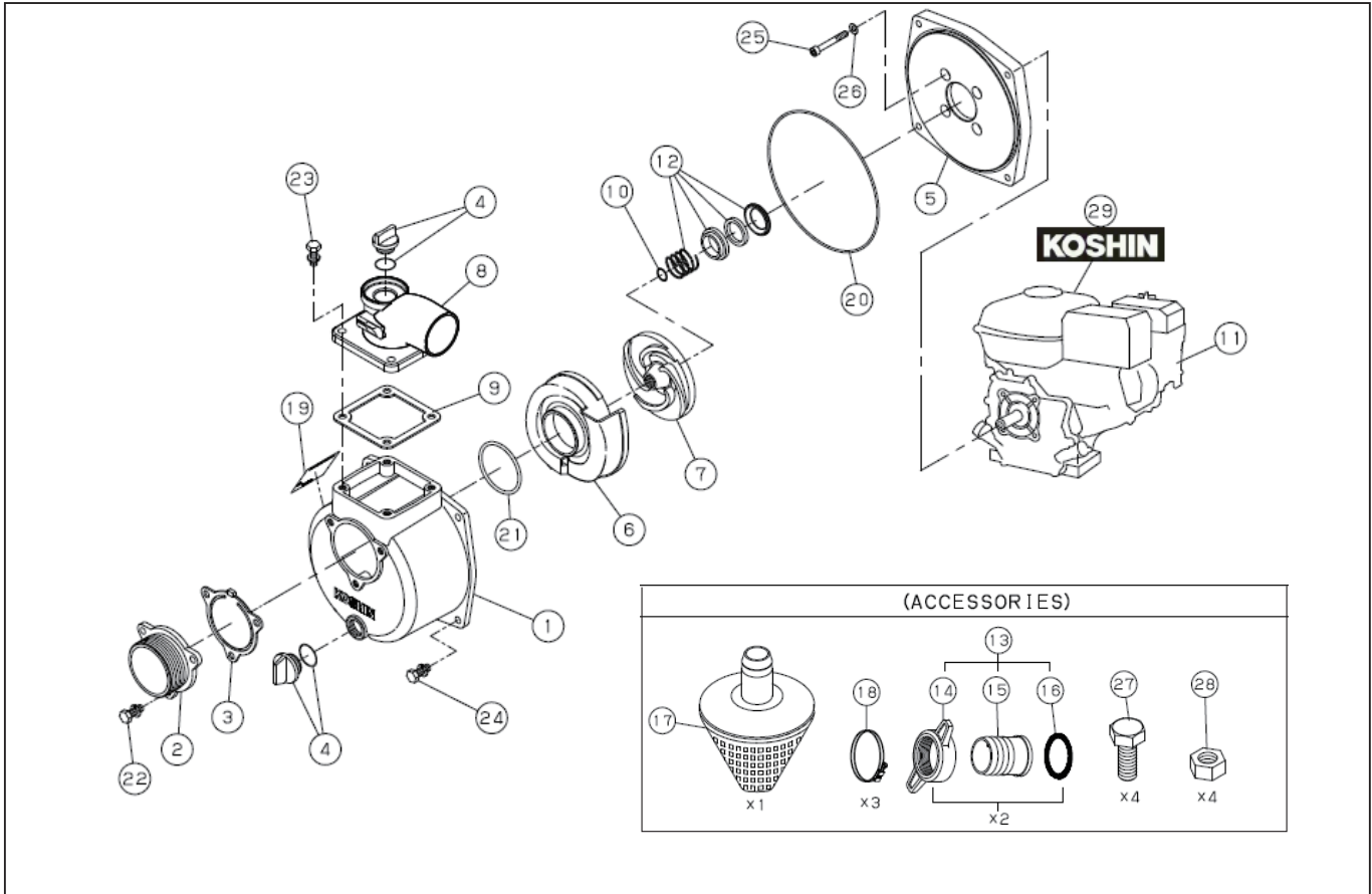
DWG No.013854403 MODEL : SEH-50X FORM : SEH-50X-BGI-0 (GX120T3)
