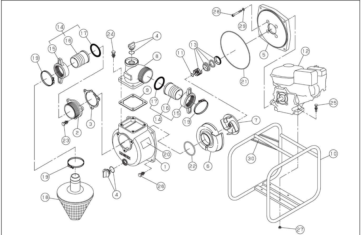
DWG No.013863601 MODEL : SEH-50X FORM : SEH-50X-BGL-0 (GX160UH2)
