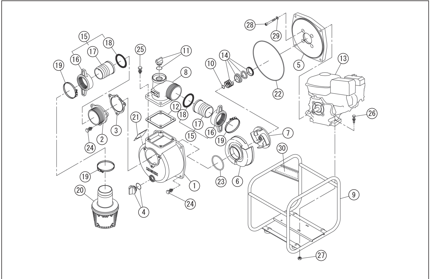
DWG No.012936201 MODEL : SEH-80P FORM : SEH-80P-BAA-0
