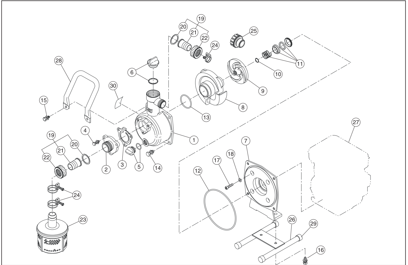
DWG No.012889503 MODEL:SEM-25E FORM:SEM-25E-BAA
