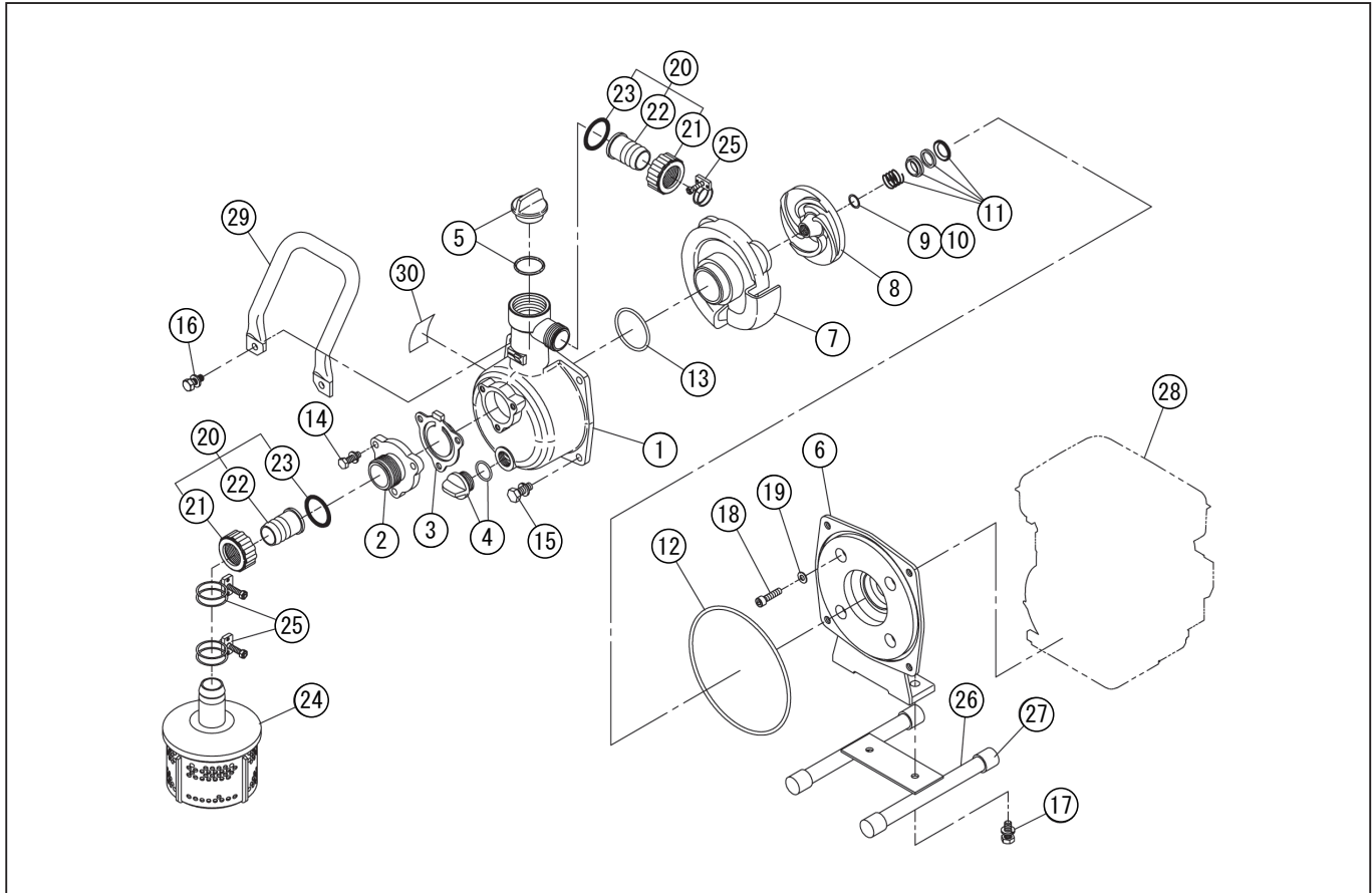
DWG No.012909320 MODELE:SEV-25L FORM:SEV-25L-BAA-4
