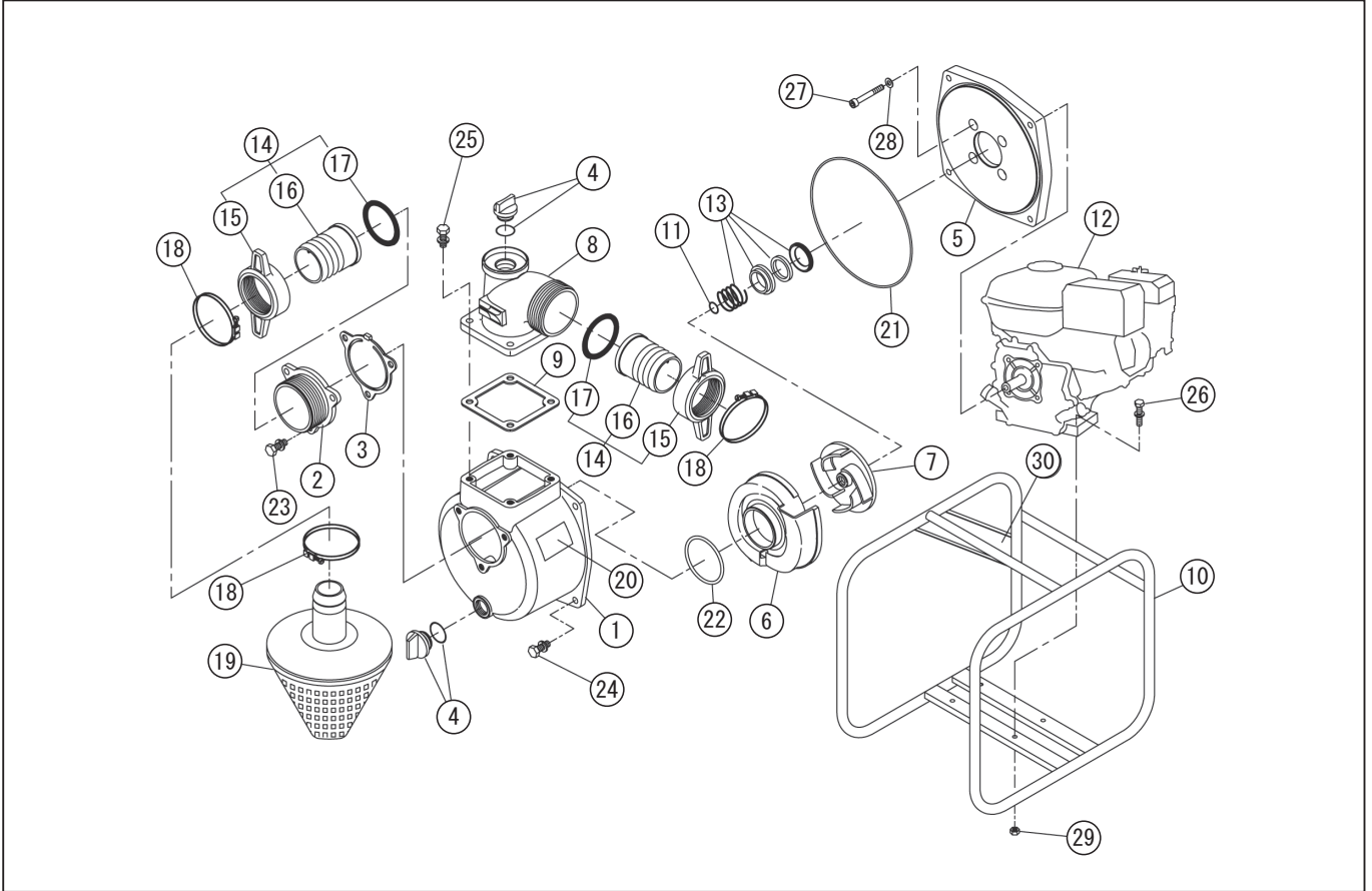
DWG No.012932901 MODEL:SEV-50X FORM:SEV-50X-BAU-0 (K180-A2)
