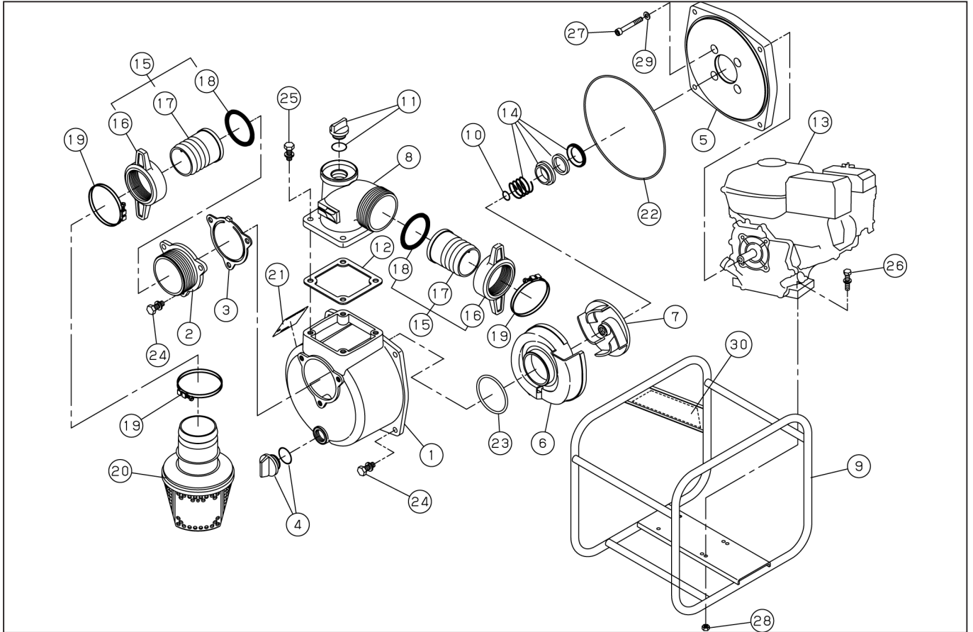
DWG No.013854801 MODEL:SEV-80E FORM:SEV-80E-BAA-0 (K210S)
