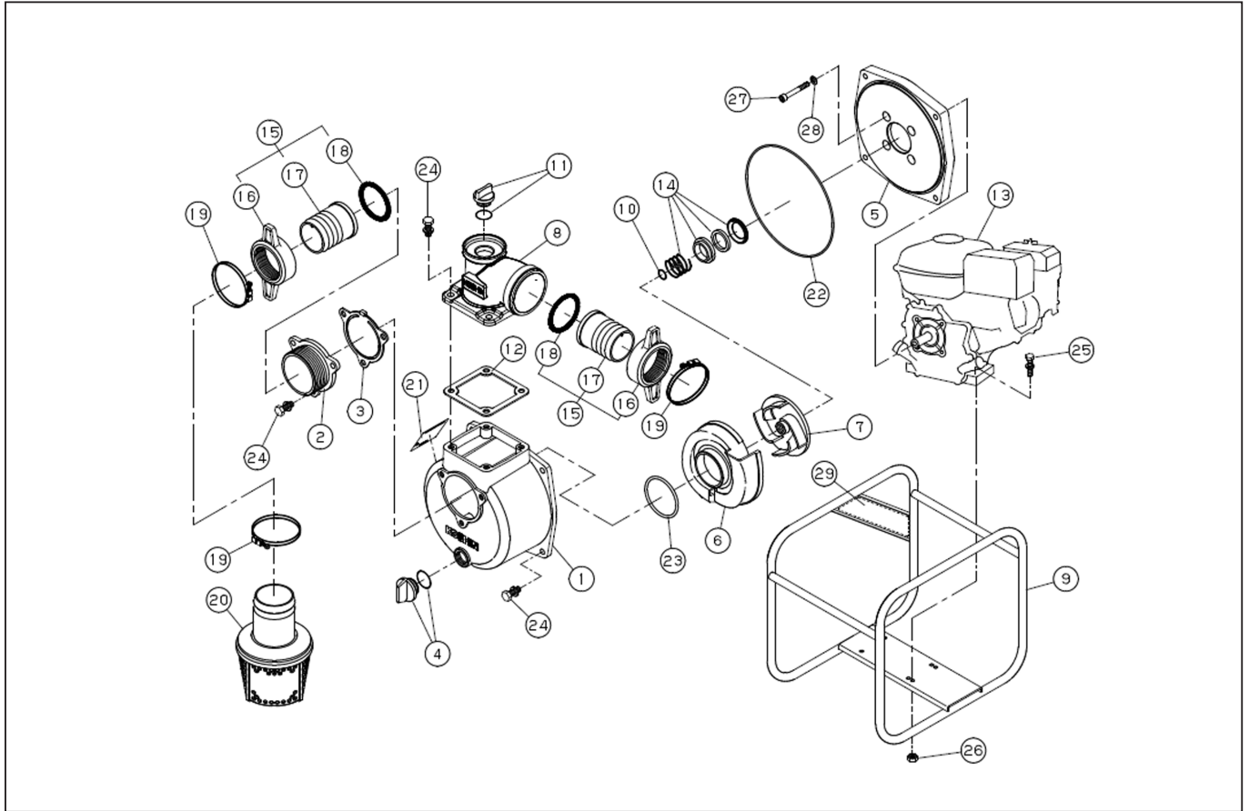
DWG No.013854805 MODEL : SEV-80E FORM : SEV-80E-BAA-2 (K210S)
