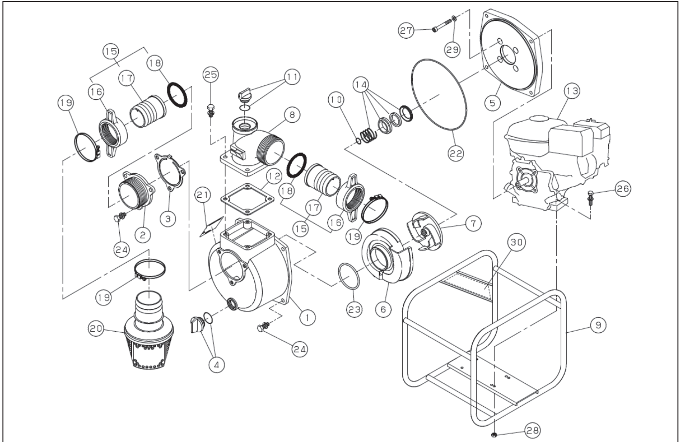
DWG No.012911815 MODEL:SEV-80X FORM:SV-80X-BAI-4
