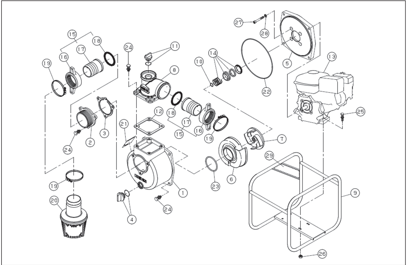
DWG No.012911819 MODEL : SEV-80X FORM : SEV-80X-BAI-6
