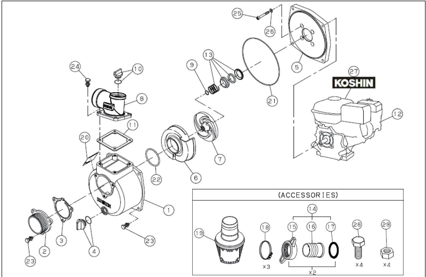
DWG No.013854305 MODEL : SEV-80X FORM : SEV-80X-BBD-1 (K180-A2)
