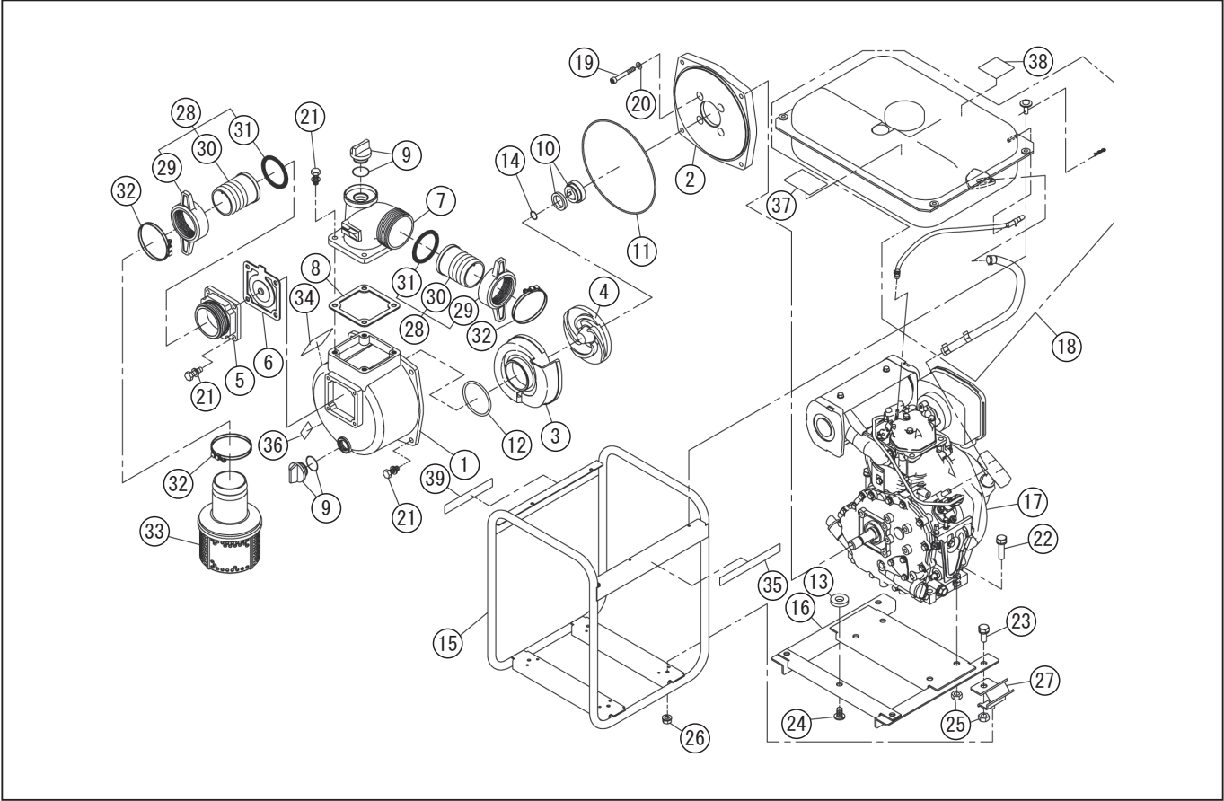
DWG No.012942805 MODELE : SEY-100D FORM : SEY-100D-BAB-1
