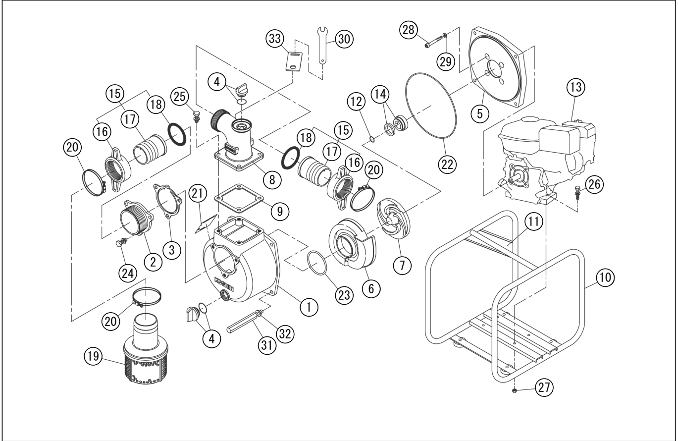
DWG No.066869602 MODELE:STH-50X FORM:STH-50X-BFH-0
