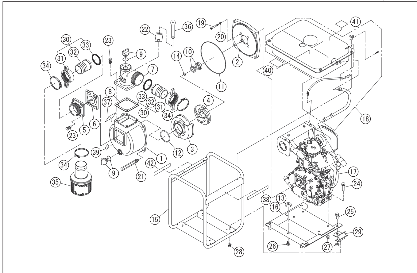
DWG No.012943104 MODELE:STY-100D FORM:STY-100D-BAB-1
