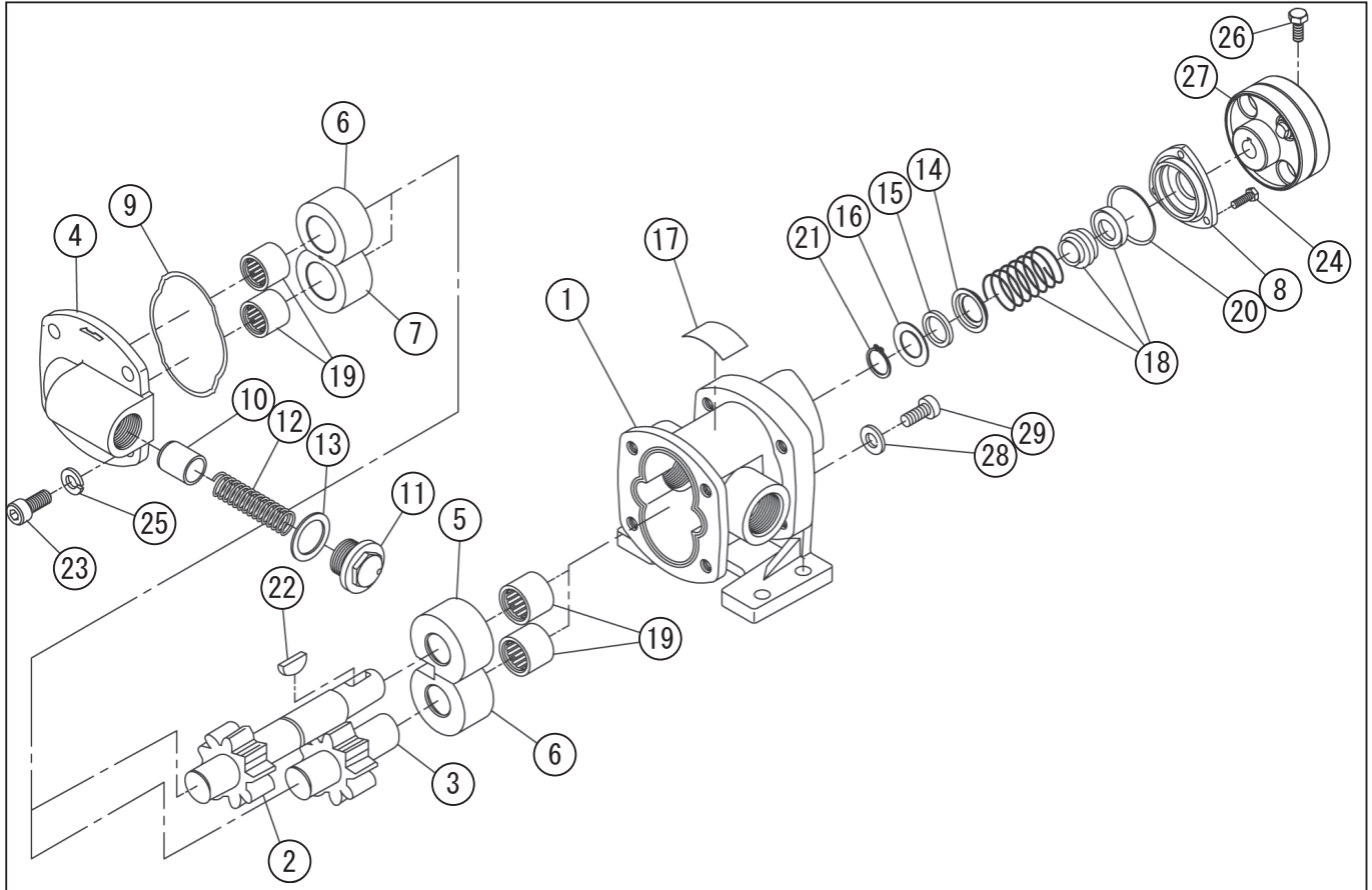
DWG No.007870811 MODEL : GL-40-10 FORM : GL-40-10-BAA-4
