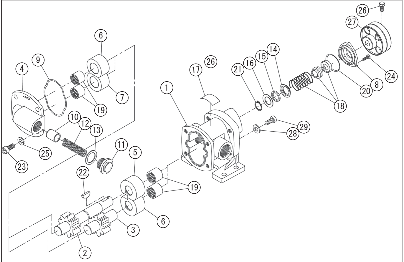
DWG No.007866116 MODEL : GL-40-5 FORM : GL-40-5-BAA-4
