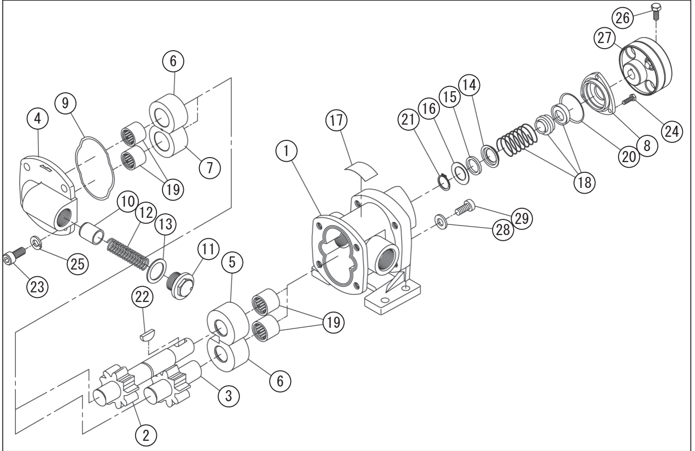
DWG No.007870910 MODEL : GL-50-10 FORM : GL-50-10-BAA-4
