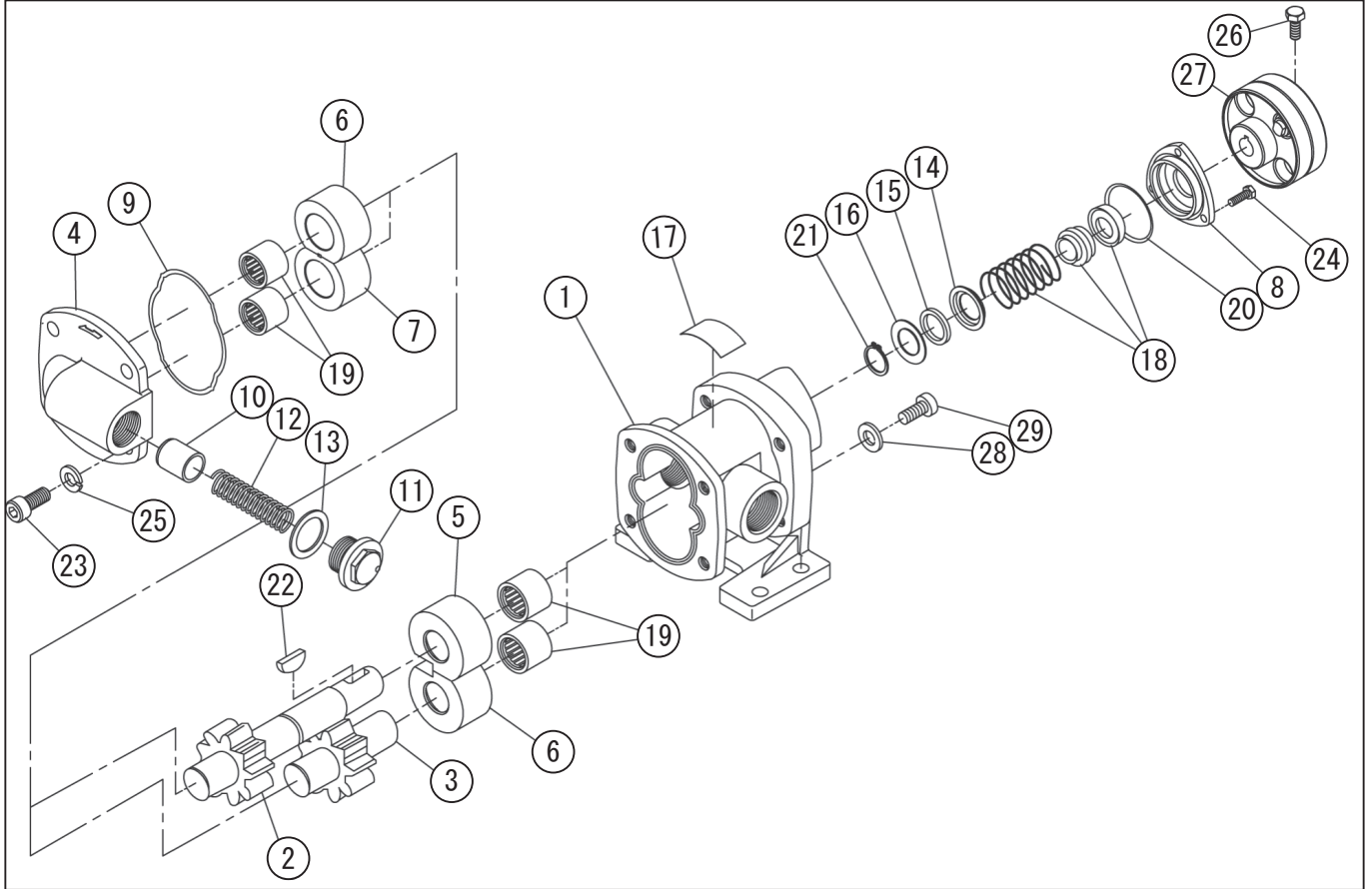
DWG No.007866216 MODEL : GL-50-5 FORM : GL-50-5-BAA-4
