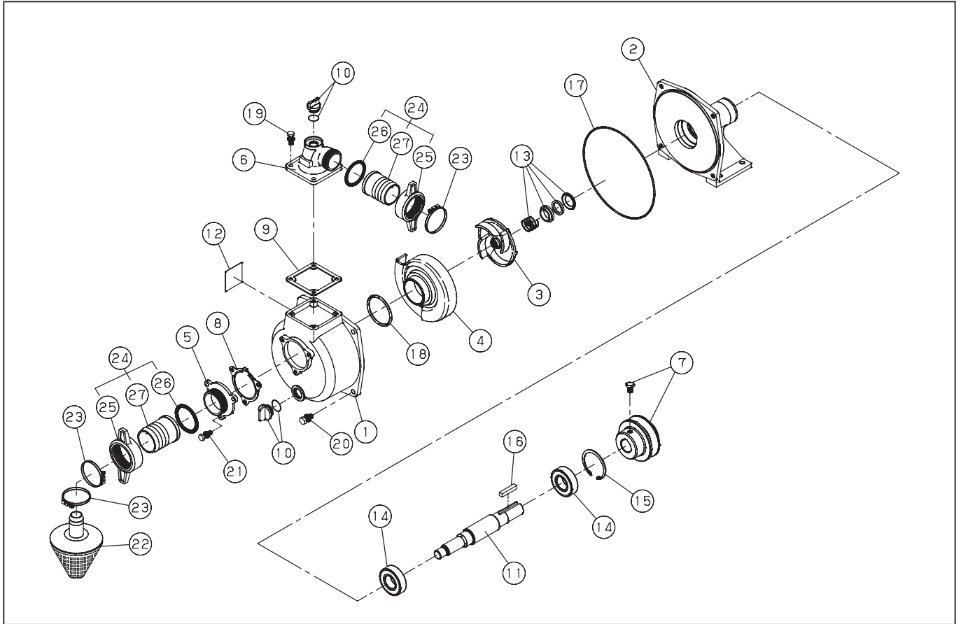
DWG No. 011973908 MODEL:SU-50H FORM:SU-50H-BAB-0
